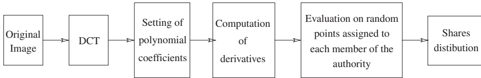
Fig. 1. Block diagram illustrating the hierarchical distribution process of the original image.
