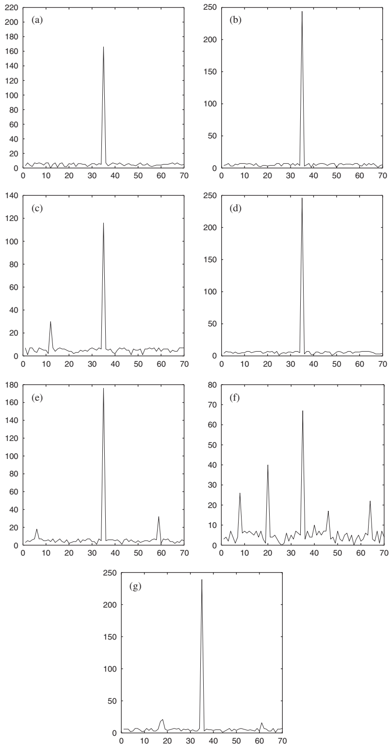
Fig. 6. Number of samples found versus signature for Lena image after: (a) additive white Gaussian noise; (b) additive uniform noise; (c) 3 \times 3 moving average; (d) Gaussian lowpass filtering; (e) scaling with a factor of 0.1; (f) rotation of 1.5^\circ ; (g) JPEG compression with quality factor equal to 25%.
