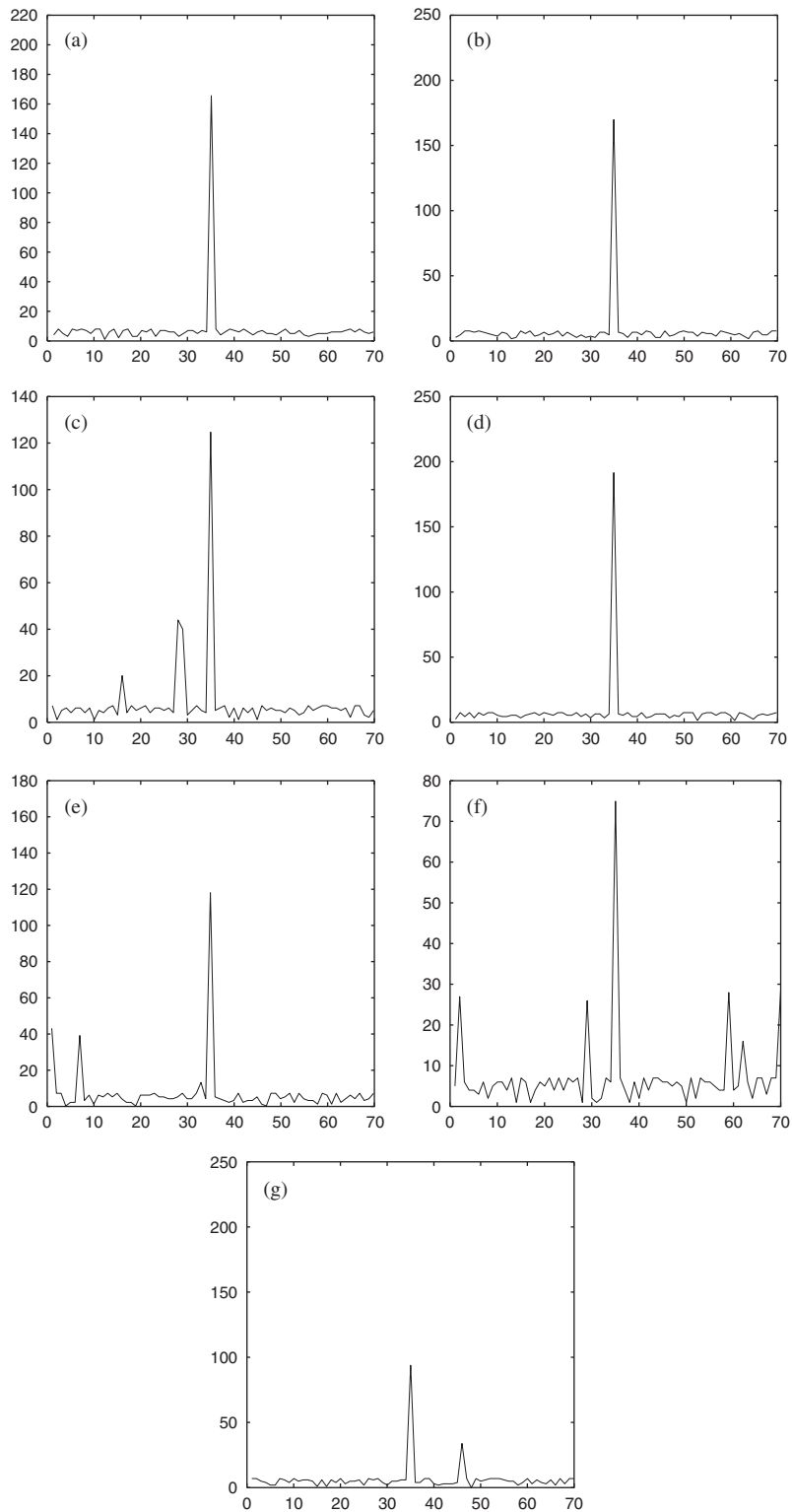
Fig. 7. Number of samples found versus signature for Baboon image after: (a) additive white Gaussian noise; (b) additive uniform noise; (c) 3 \times 3 moving average; (d) Gaussian lowpass filtering; (e) scaling with a factor of 0.1; (f) rotation of 1.5^\circ ; (g) JPEG compression with quality factor equal to 25%.
