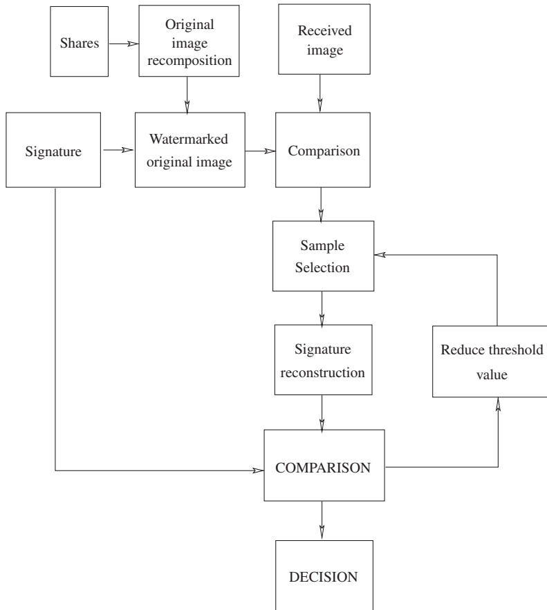
Fig. 3. Block diagram of the watermark reconstruction process.
