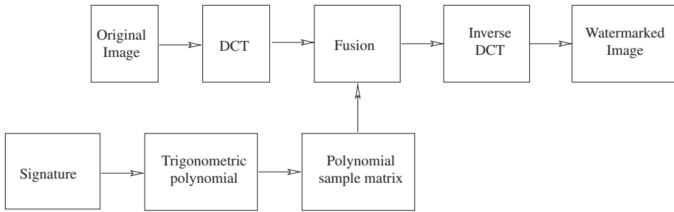
Fig. 2. Block diagram showing the various steps occurring in the watermark embedding process.
